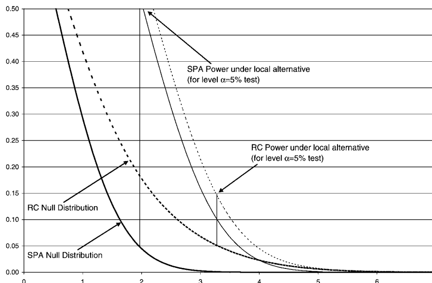
Figure 1. (One minus) The cdfs for the Test Statistics T_n^{RC} and T_n^{SPA} Under the Null Hypothesis, \mu_1 = \mu_2 = 0 , and the Local Alternative, \mu_2 = 2/\sqrt{n} > 0 . [ \text{---} 1 - F_0(x) ; \text{- - -} 1 - F_1(x) ; \text{— — —} 1 - G_0(x) ; \text{— — —} 1 - G_1(x) .] Studentization improves the power from about 15% to about 53%.
