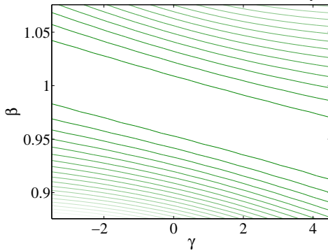
Figure 6.1: This figure contains a plot of the GMM objective function using the 2-step estimator (top panels) and the CUE (bottom panels). The objective is very steep along the \beta axis but nearly flat along the \gamma axis. This indicates that \gamma is not well identified.
