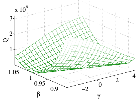
Figure 6.1: This figure contains a plot of the GMM objective function using the 2-step estimator (top panels) and the CUE (bottom panels). The objective is very steep along the \beta axis but nearly flat along the \gamma axis. This indicates that \gamma is not well identified.
