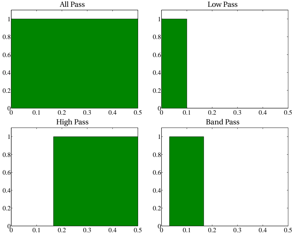
Figure 4.10: These four panels depict the gain functions from a set of ideal filters . The all-pass filter allows all frequencies through. The low-pass filter cuts off at \frac{1}{10} . The high-pass cuts off below \frac{1}{6} and the band-pass filter cuts off below \frac{1}{32} and above \frac{1}{6} .
