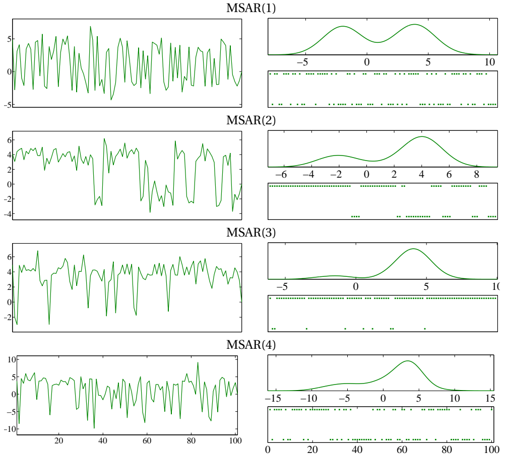
Figure 4.13: The four panels of this figure contain simulated data generated by the 4 Markov switching processes described in the text. In each panel, the large subpanel contains the generated data, the top right subpanel contains a kernel density estimate of the unconditional density and the bottom right subpanel contains the time series of the state values (high points correspond to the high state).
