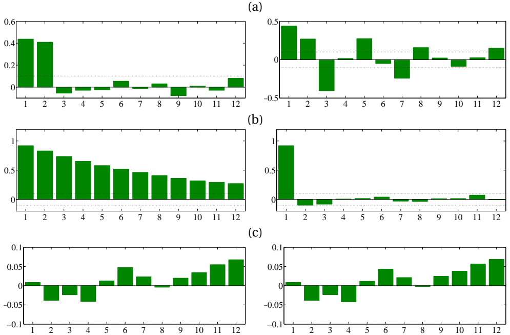
Figure 4.15: The ACF and PACF of three stochastic processes. Use these to answer question 4.9.
