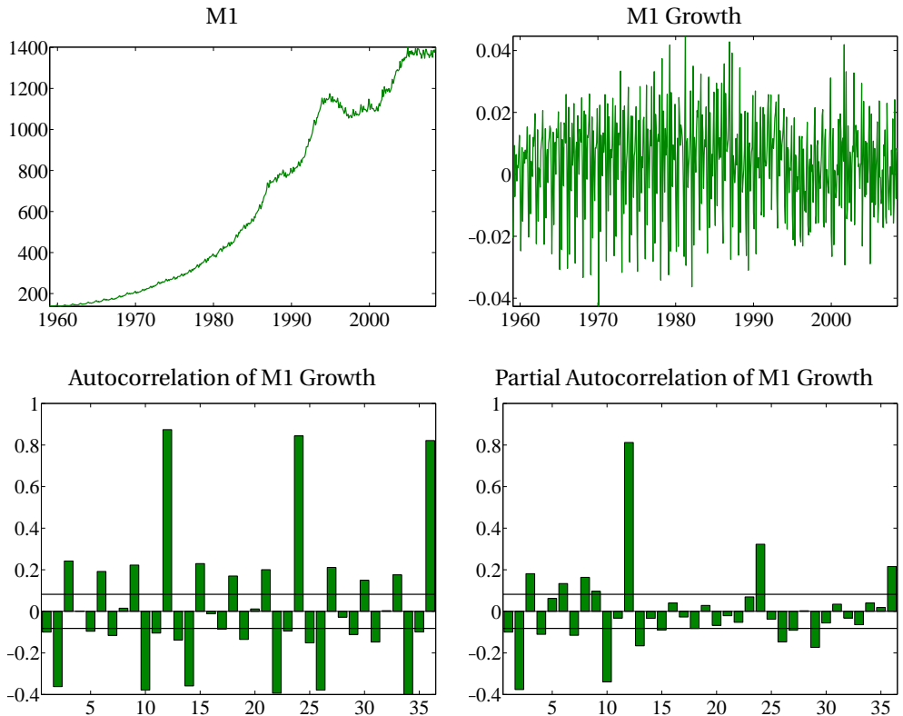
Figure 4.7: Plot of the money supply (M1), M1 growth (log differences), and the sample autocorrelogram and sample partial autocorrelogram of M1 growth. There is a clear seasonal pattern at 12 months which appears consistent with a seasonal ARMA(1,1).
