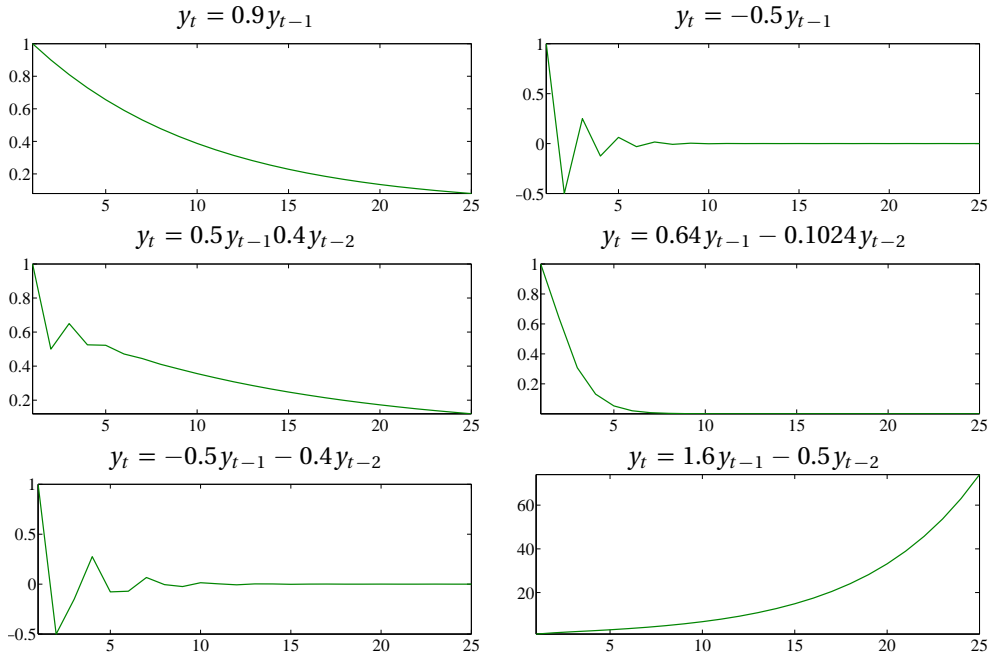
Figure 4.1: These six plots correspond to the dynamics of the six linear homogeneous systems described in the text. All processes received a unit shock at t = 1 ( x_1 = 1 ) and no other shocks ( x_j = 0, j \neq 1 ). Pay close attention to the roots of the characteristic polynomial and the behavior of the system (exponential decay, oscillation and/or explosion).
