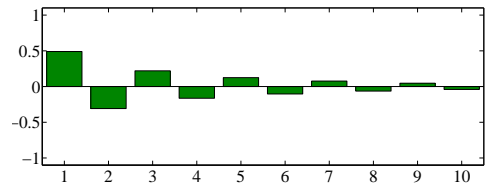
Figure 4.4: Autocorrelation function and partial autocorrelation function for 4 processes. Note the difference between how the ACF and PACF respond in AR and MA models.
