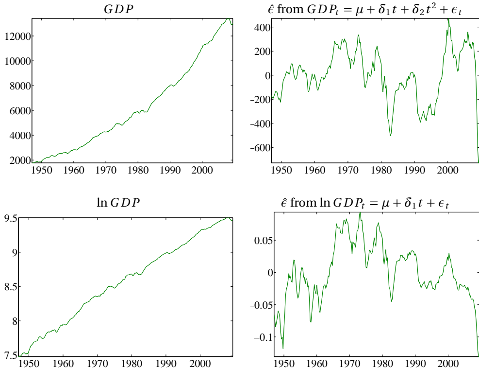
Figure 4.8: Two time trend models are presented, one on the levels of GDP and one on the natural log. Note that the detrended residuals are still highly persistent. This is a likely sign of a unit root.
