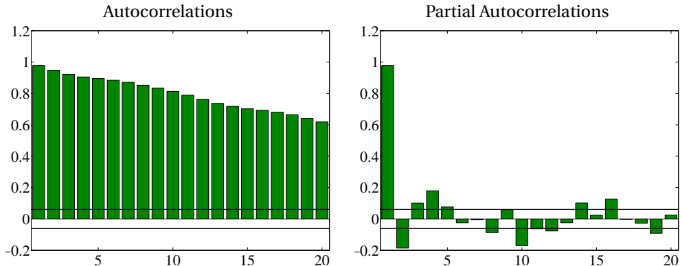
Figure 4.6: These for pictures plot the first 20 autocorrelations (left) and partial autocorrelations (right) of the VWM (top) and the Baa-Aaa spread (bottom). Approximate standard errors, assuming homoskedasticity, are in parenthesis.
