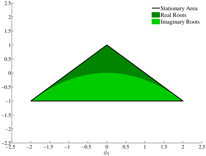
Figure 4.2: The triangular region corresponds to the values of the parameters in the AR(2) y_t = \phi_1 y_{t-1} + \phi_2 y_{t-2} + \epsilon_t . The dark region corresponds to real roots and the light region corresponds to imaginary roots.
