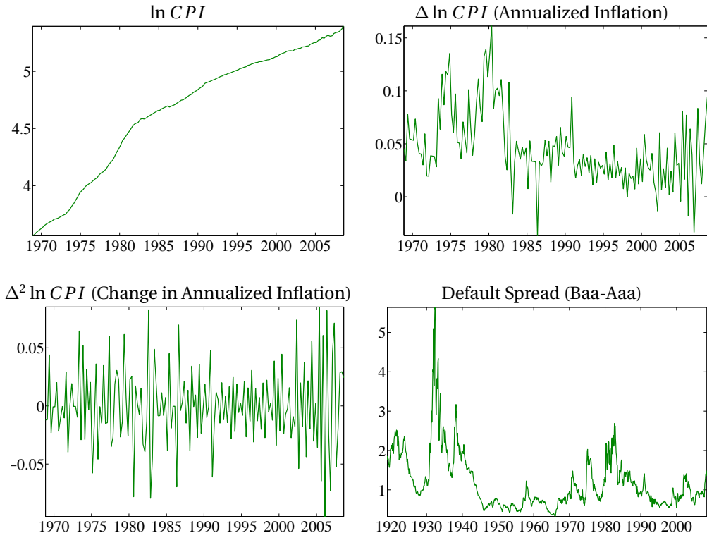
Figure 4.9: These four panels plot the log consumer price index ( \ln CPI ), \Delta \ln CPI , \Delta^2 \ln CPI and the default spread. Both \Delta^2 \ln CPI and the default spread reject the null of a unit root.
