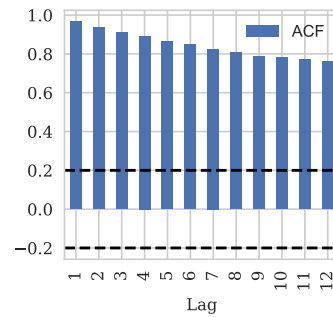
Figure 4.16: Plots for question 2(b).
