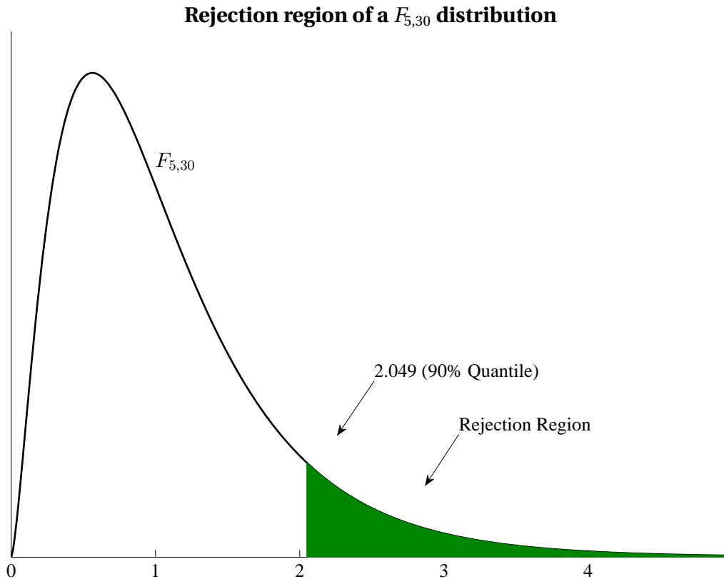
Figure 3.3: Rejection region for a F_{5,30} distribution when using a test with a size of 10%. If the null hypothesis is true, the test statistic should be relatively small (would be 0 if exactly true). Large test statistics lead to rejection of the null hypothesis. In this example, a test statistic with a value greater than 2.049 would lead to a rejection of the null at the 10% level.
