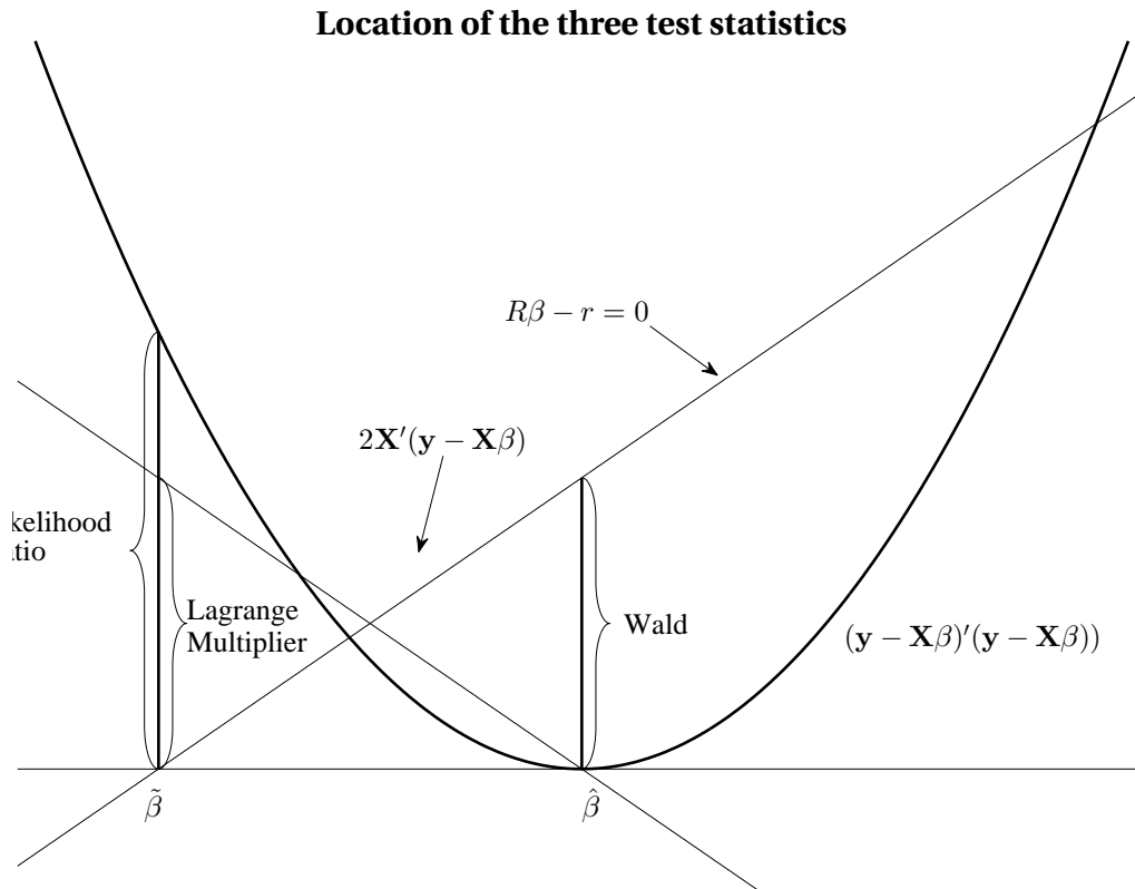
Figure 3.4: Graphical representation of the three major classes of tests. The Wald test measures the magnitude of the constraint, R\hat{\beta} - r , at the OLS parameter estimate, \hat{\beta} . The LM test measures the magnitude of the score at the restricted estimator ( \tilde{\beta} ) while the LR test measures the difference between the SSE at the restricted estimator and the SSE at the unrestricted estimator. Note: Only the location of the test statistic, not their relative magnitudes, can be determined from this illustration.
