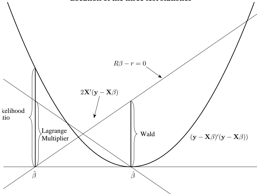
Figure 3.4: Graphical representation of the three major classes of tests. The Wald test measures the magnitude of the constraint, \mathbf{R}\boldsymbol{\beta} - r , at the OLS parameter estimate, \hat{\boldsymbol{\beta}} . The LM test measures the magnitude of the score at the restricted estimator ( \tilde{\boldsymbol{\beta}} ) while the LR test measures the difference between the SSE at the restricted estimator and the SSE at the unrestricted estimator. Note: Only the location of the test statistic, not their relative magnitudes, can be determined from this illustration.
