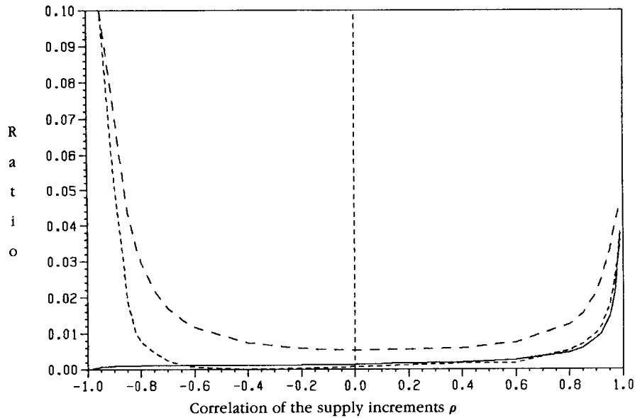
Figure 4 The ratio of the value of technical analysis and expected time 2 investment of the technician, \pi/E(d_{t_2}, P_1 | \mathcal{E}_0) , shown as a function of \rho , the correlation of the supply increments x_1 and x_2 . The solid line represents the case in which V_1^2 = V_2^2 = 226 , the short-dashed line the case in which V_1^2 = 113 and V_2^2 = 226 , and the long-dashed line the case in which V_1^2 = 226 and V_2^2 = 113 . The values of the remaining parameters are set equal to the base values shown in Section A of Appendix C.
