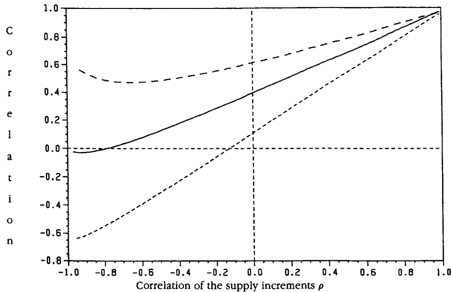
Figure 5 The unconditional correlation in price changes \text{corr}(P_2 - P_1, u - P_2 | \mathcal{Z}_0) , as a function of \rho , the correlation between supply increments x_1 and x_2 . The solid line represents the case in which V_1^2 = V_2^2 = 226 , the short-dashed line the case in which V_1^2 = 113 and V_2^2 = 226 , and the long-dashed line the case in which V_1^2 = 226 and V_2^2 = 113 . The values of the remaining parameters are set equal to the base values shown in Section A of Appendix C.
